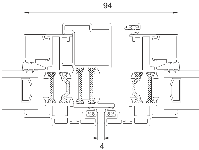
Meeting Stile
