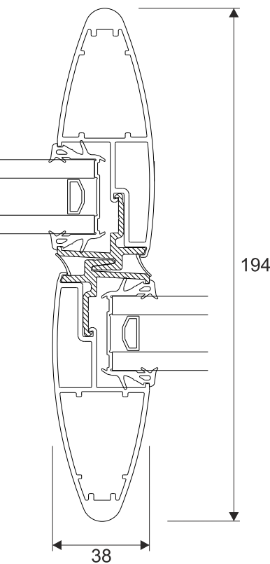
Heavy Duty Interlock
