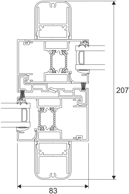
Double Heavy Duty Interlock
